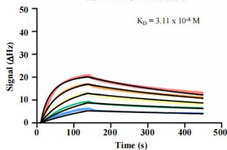
Beta RBD-ACE2 interaction
